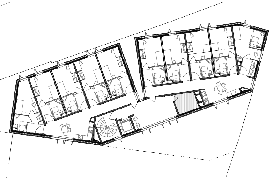
Plan R+3
