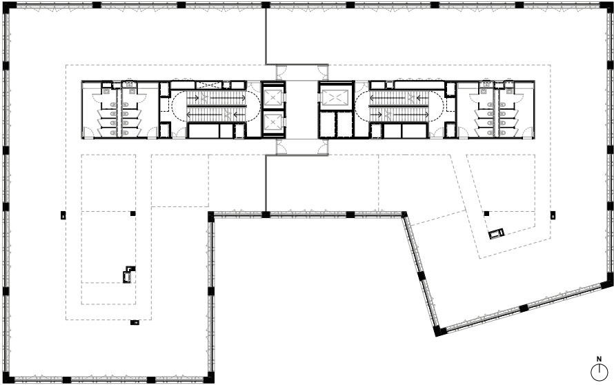
Plan R+3
