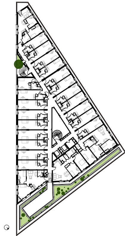
Plan R+4
