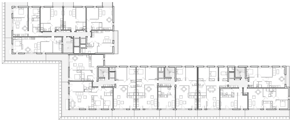
Plan R+1
